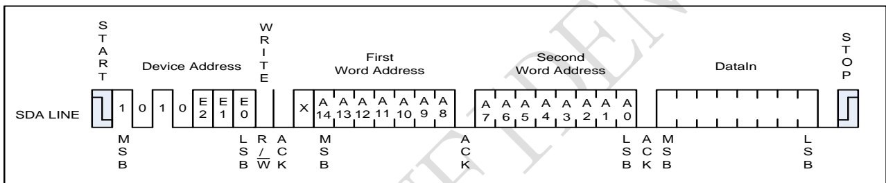
Figure 5-1 Byte Write
